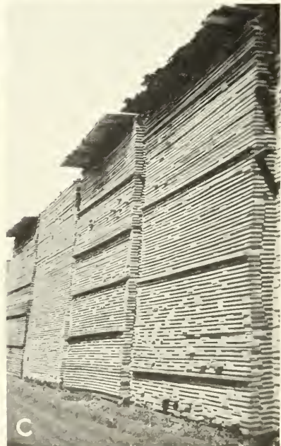
Rear alleys; bad and good practice: A, Poor piling of yard lumber. Overhanging ends, inadequate sticketing, insufficient and improper foundations, weeds, and a narrow and obstructed alley all cause degrade, with its resulting loss; B, an adequate rear alley, wide and well-kept except for the few scattered stickers. All the piles are set up properly (box piled), and the sanitation is good; C, one side of a well-appearing rear alley. The stock is piled without overhanging ends (box piling), a desirable feature. Three or four rear pile ends, in addition, have drip boards. On the other hand, higher foundations are desirable
